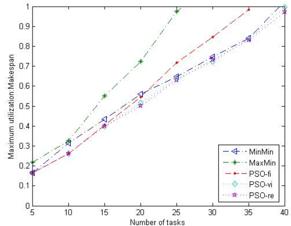
Fig. 2 A comparison of partitioning methods with light tasks partitioned upon 4 processors.
