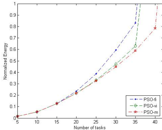
Fig. 8 A comparison among PSO-fi, PSO-vi, and PSO-m techniques with light tasks partitioned upon 4 processors.
