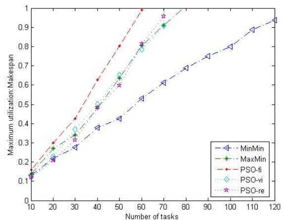
Fig. 3 A comparison of partitioning methods with light tasks partitioned upon 10 processors.
