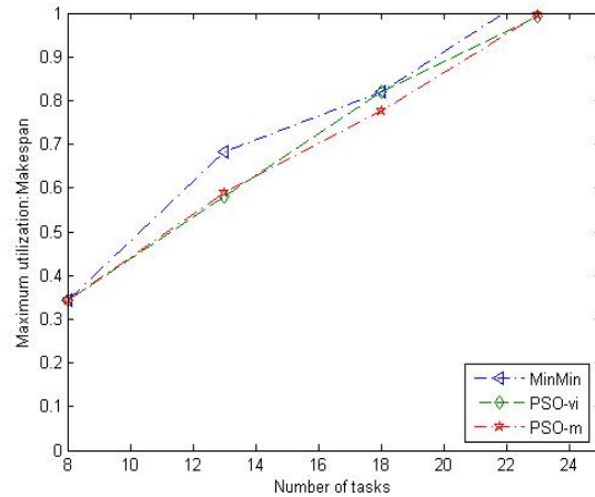
Fig. 6 A comparison among Min-min, PSO-vi, and PSO-m techniques with medium tasks partitioned upon 8 processors.
