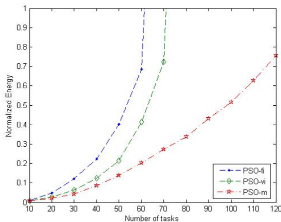
Fig. 9 A comparison among PSO-fi, PSO-vi, and PSO-m techniques with light tasks partitioned upon 10 processors.
