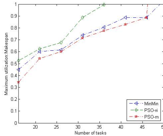
Fig. 7 A comparison among Min-min, PSO-vi, and PSO-m techniques with medium tasks partitioned upon 16 processors.
