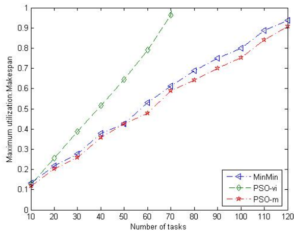
Fig. 5 A comparison among Min-min, PSO-vi, and PSO-m techniques with light tasks partitioned upon 10 processors.
