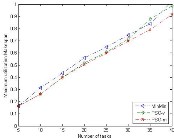
Fig. 4 A comparison among Min-min, PSO-vi, and PSO-m techniques with light tasks partitioned upon 4 processors.
