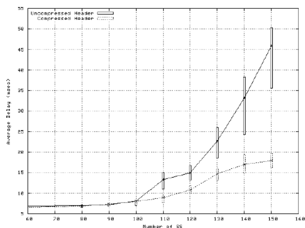
Figure 13: Average VoIP Packet Delay
